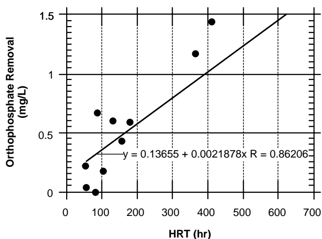
Figure 4-8. Retention Time vs. Orthophosphate Removal (mg/l)
