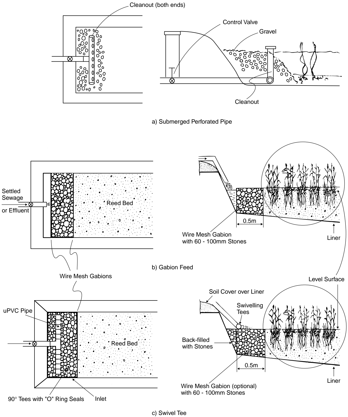
Figure 6-2. Examples of constructed wetland inlet designs
