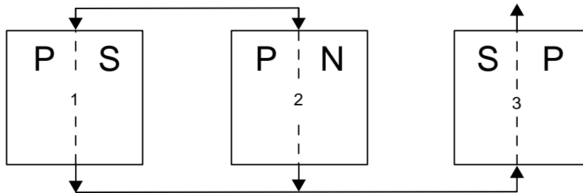
Figure 8-6. Schematic of Minoa, NY, VSB system
