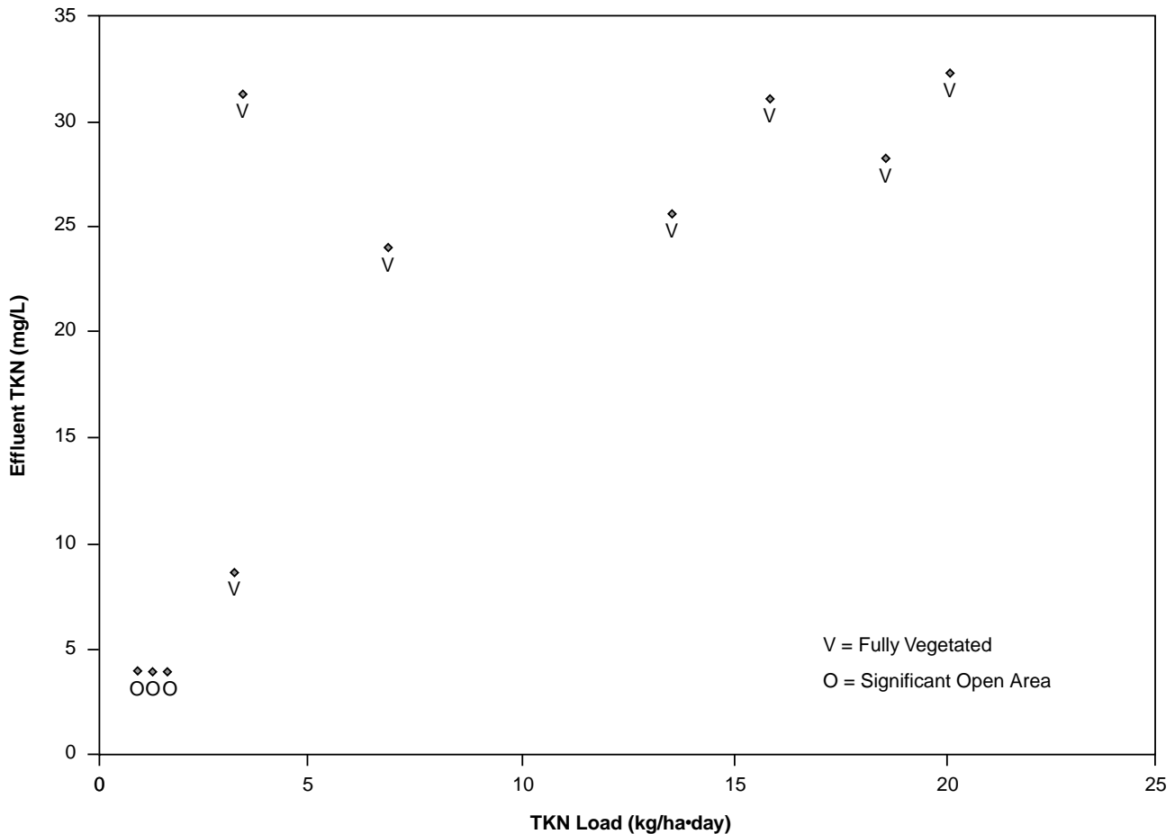
Figure 4-5. Effluent TKN vs. TKN loading
