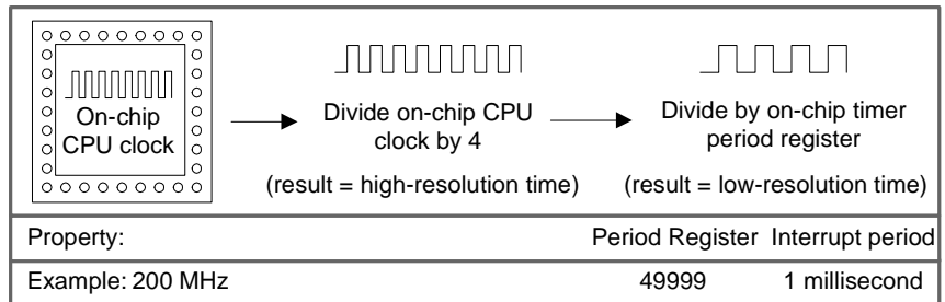
Figure 4–8 CLK Module Properties
