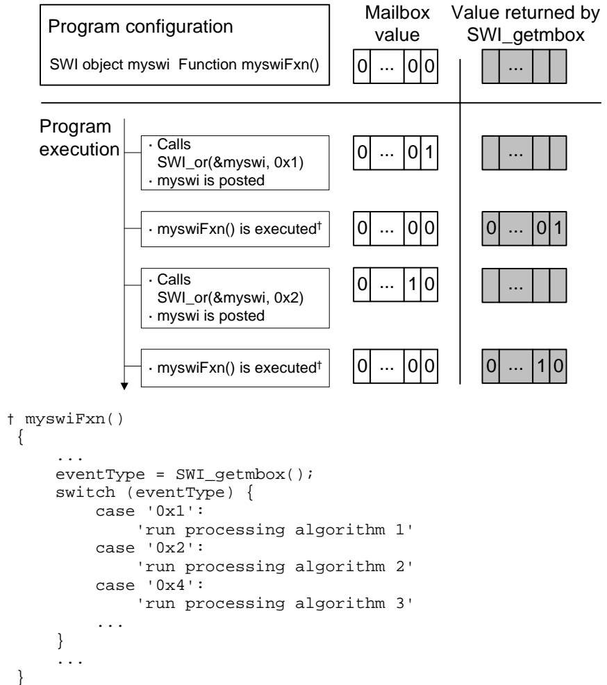
Figure 4–3 Using SWI_or to Post an SWI.
