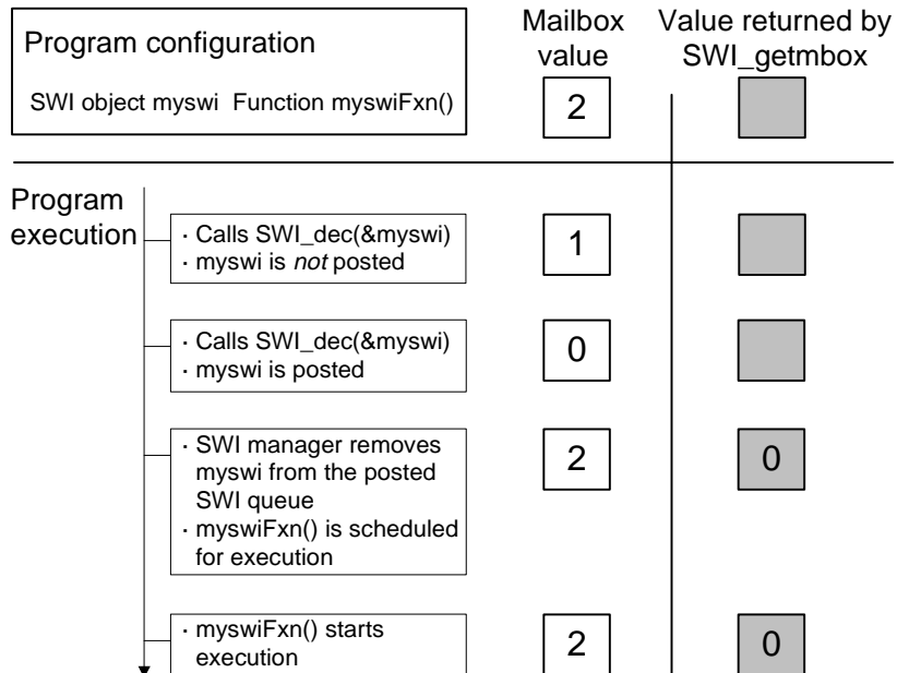
Figure 4–4 Using SWI_dec to Post an SWI
