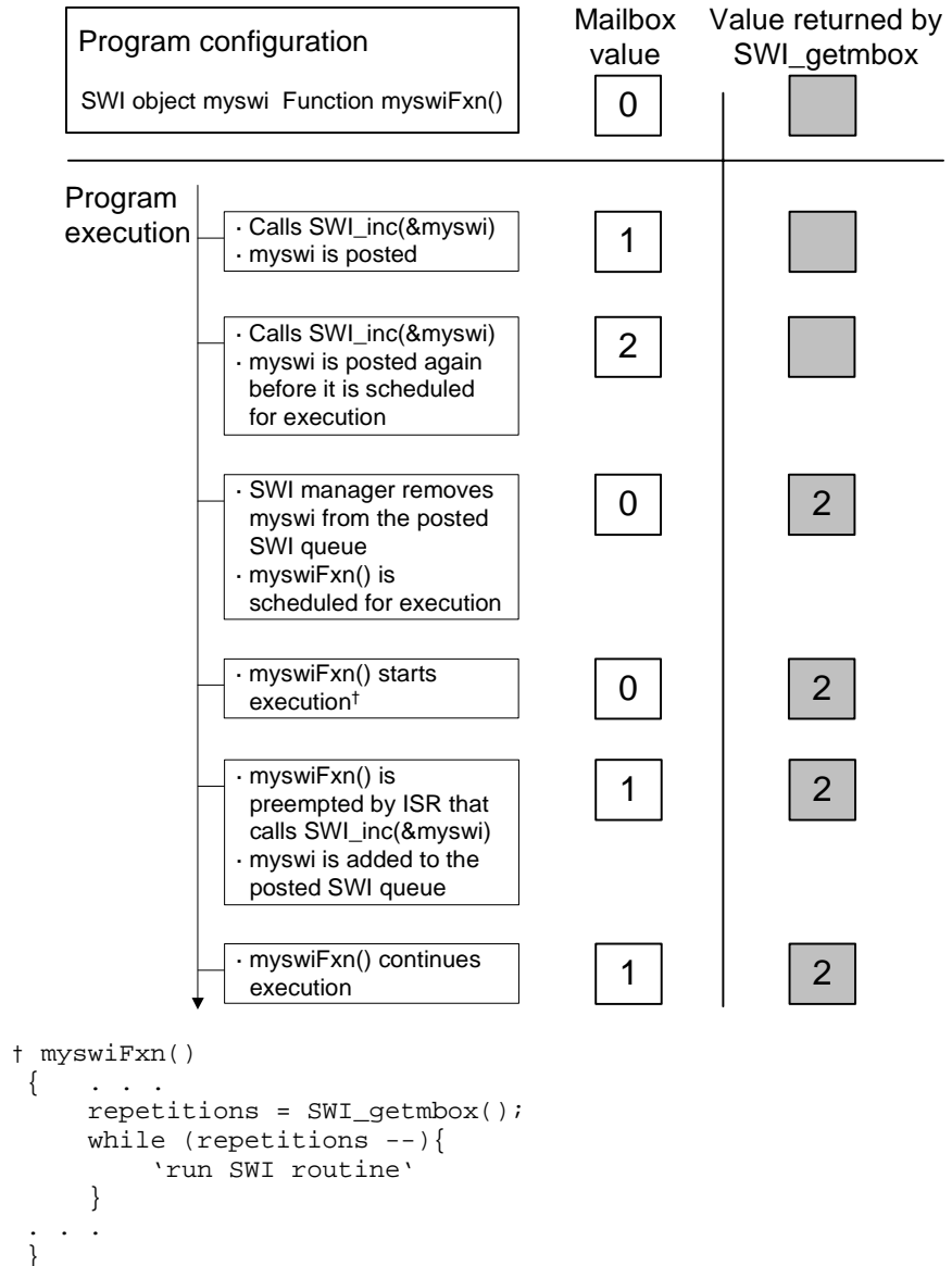
Figure 4–1 Using SWI_inc to Post an SWI
