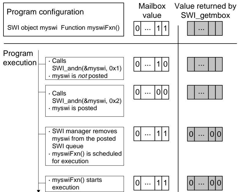
Figure 4–2 Using SWI_andn to Post an SWI
