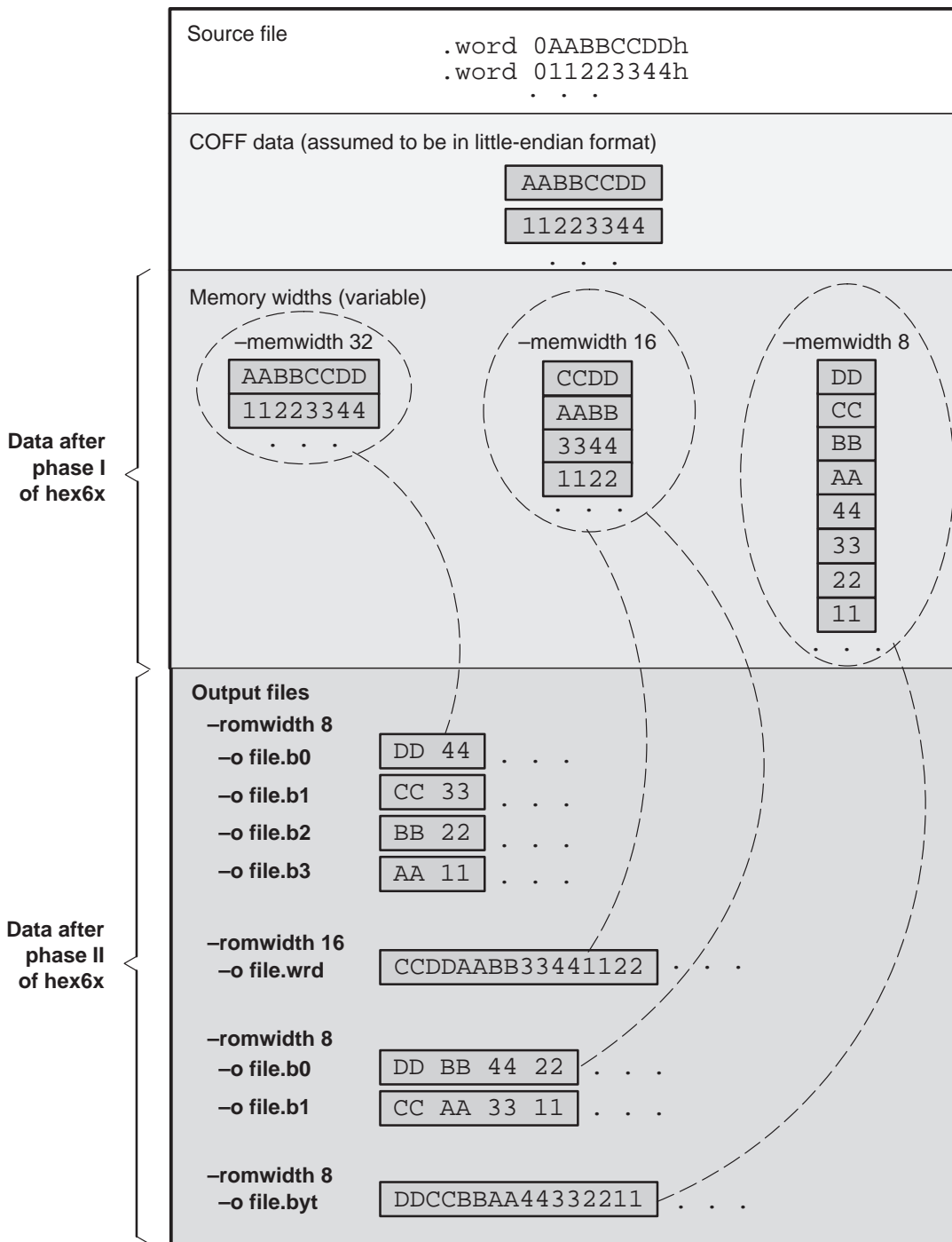
Figure 10–4. Data, Memory, and ROM Widths
