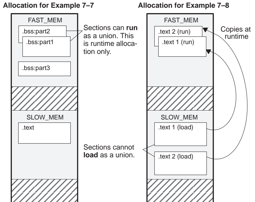
Figure 7–4. Memory Allocation Shown in Example 7–7 and Example 7–8
