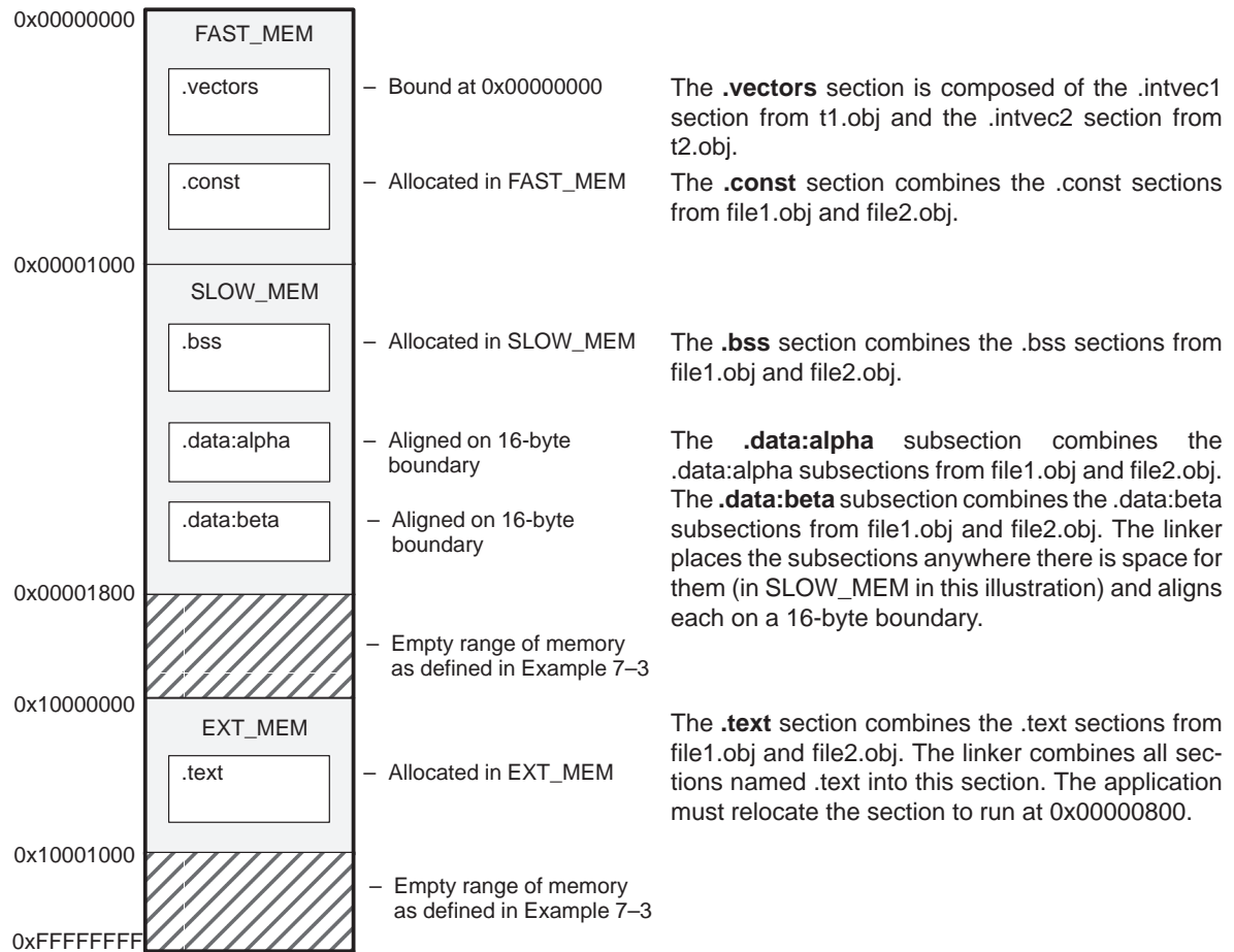
Figure 7–2. Section Allocation Defined by Example 7–4
