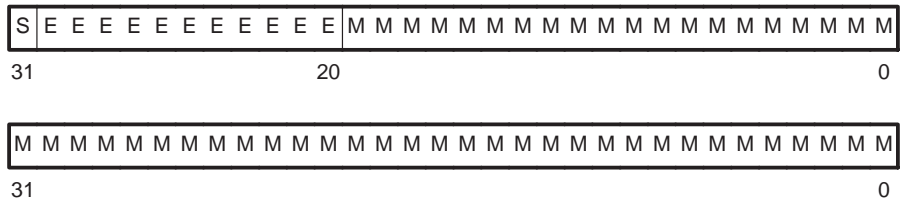
Figure 4–5. Double-Precision Floating-Point Format
