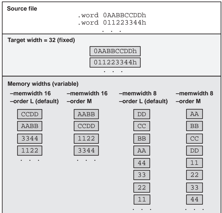
Figure 10–5. Varying the Word Order
