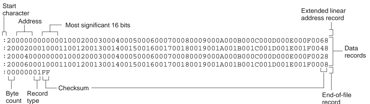
Figure 10–8. Intel Hexadecimal Object Format
