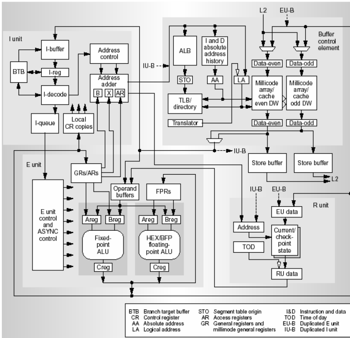
Figure 2. Diagram of the G5 microprocessor.
