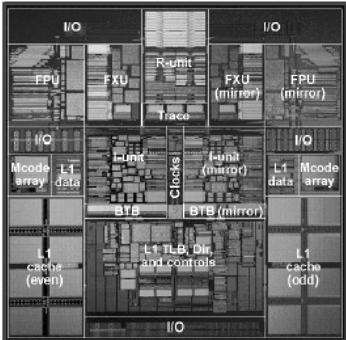
Figure 1. Micrograph of the IBM S/390 G5 microprocessor.
