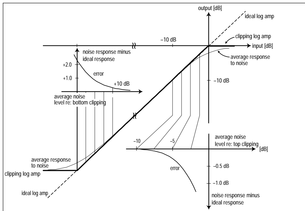
Figure D. In its center, this graph shows three curves: the ideal log amp behavior, that of a log amp that clips at its maximum and minimum extremes, and the average response to noise subject to that clipping. The lower right plot shows, on expanded scales, the error in average noise response due to clipping at the positive extreme. The average level should be kept 7 dB below the clipping level for an error below 0.1 dB. The upper left plot shows, with an expanded vertical scale, the corresponding error for clipping against the bottom of the scale. The average level must be kept 14 dB above the clipping level for an error below 0.1 dB.
