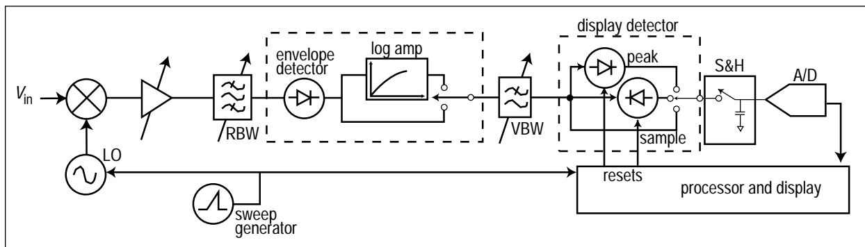
Figure A. Simplified spectrum analyzer block diagram
