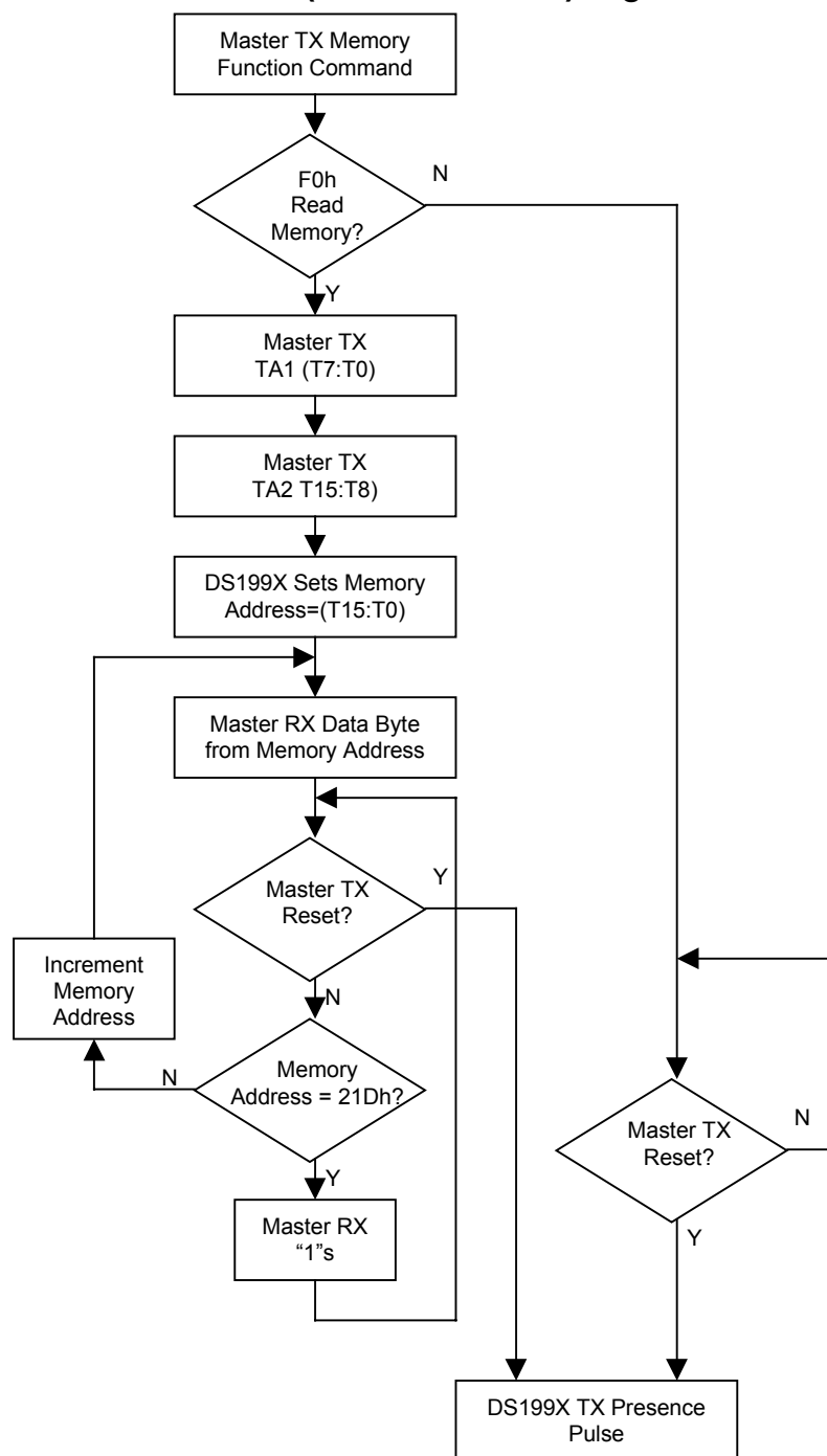
DS1994 READ MEMORY FLOW (DATA SHEET) Figure 1
