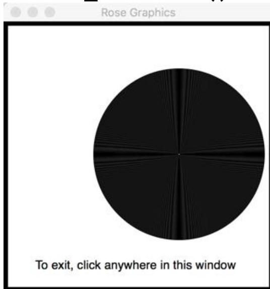
draw_circles3()
