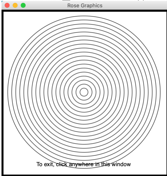
draw_circles1()
